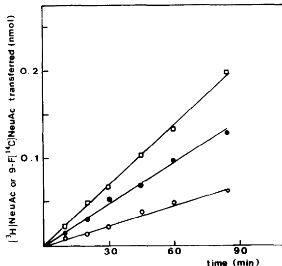
Fig.3. Incorporation of N -[ 3 H]acetylneuraminic acid and 9-fluoro- N -[ 14 C]acetylneuraminic acid in \alpha_1 -acid glycoprotein by rat liver sialyltransferase. 32.5 \mu M CMP- N -[ 3 H]acetylneuraminic acid ( 6 \times 10^5 dpm) (□—□), 65 \mu M CMP-9-fluoro- N -[ 14 C]acetylneuraminic acid ( 6 \times 10^5 dpm) (○—○), 130 \mu M CMP-9-fluoro- N -[ 14 C]acetylneuraminic acid ( 1.2 \times 10^6 dpm) (●—●). After the indicated times, aliquots were removed from incubations and acid-precipitable radioactivity was determined.
