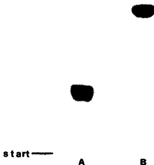
Fig.2. Autoradiography of a thin-layer chromatogram of purified 9-fluoro- N -[ 14 C]acetylneuraminic acid (A) and CMP-9-fluoro- N -[ 14 C]acetylneuraminic acid (B) run in solvent B. Authentic N -acetylneuraminic acid and its corresponding sugar nucleotide both have a slightly lower mobility as compared to the 9-fluoro derivatives.
