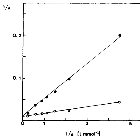
Fig.1. Kinetics of N -[ 3 H]acetylneuraminic acid and 9-fluoro- N -[2- 14 C]acetylneuraminic acid activation. Initial velocities are plotted as functions of N -[ 3 H]acetylneuraminic acid concentration (○—○) and 9-fluoro- N -[ 14 C]acetylneuraminic acid concentration (●—●). Product formation was measured by the radiochemical test. Velocity is expressed as product formed within 10 min in 0.1 ml at a protein concentration of 0.135 mg. The calculation of K_m for N -acetylneuraminic acid as substrate afforded a second plot with a reduced enzyme concentration (not shown).
